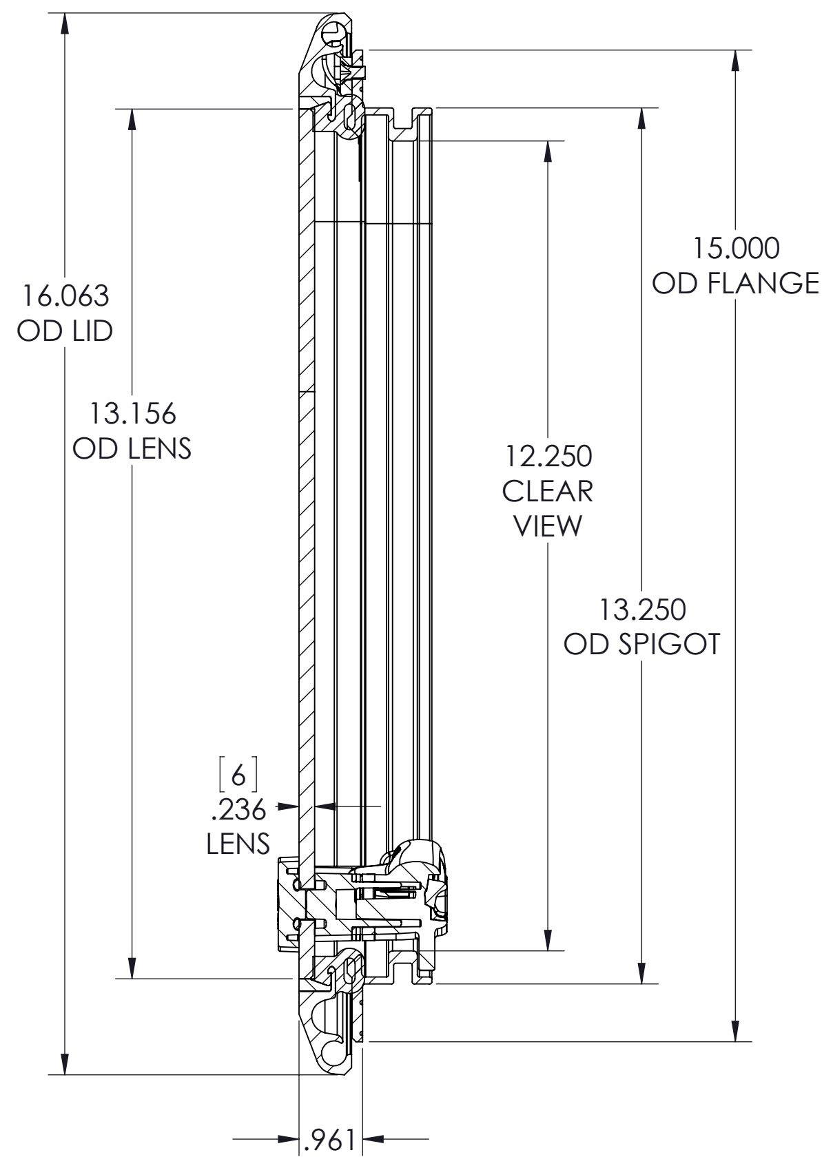
SECTION B-B
